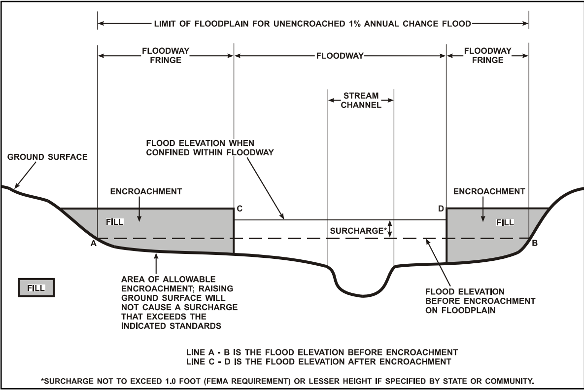
Figure 3 – Floodway Schematic
